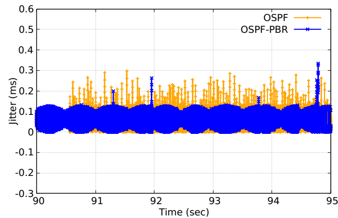
Figure 6. Jitter comparison in OSPF and OSPF with PBR module.
