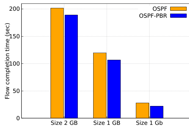
Figure 7. Flow completion time in OSPF and OSPF with PBR module.
