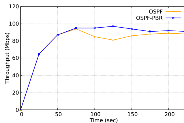
Figure 5. Throughput comparison in OSPF and OSPF with PBR module.
