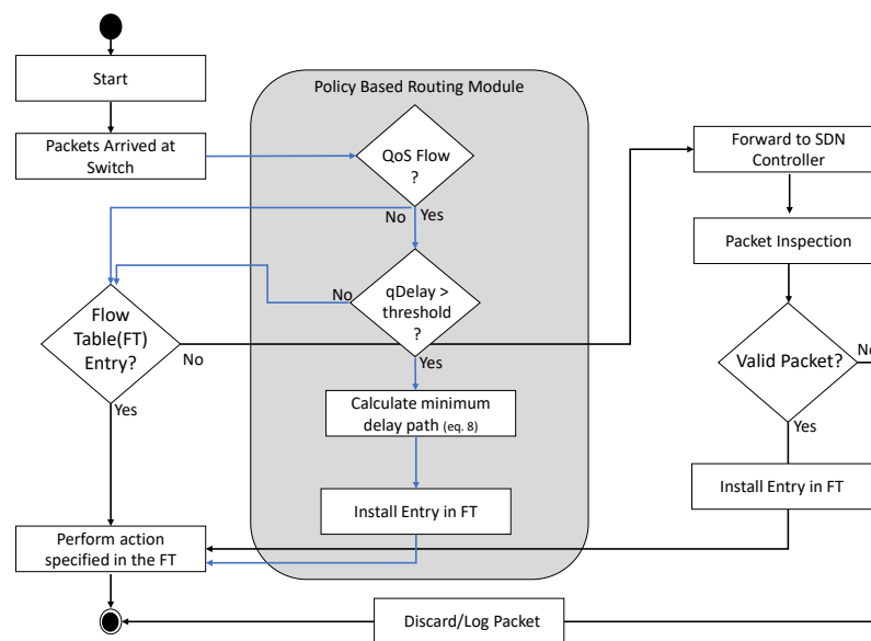
Figure 1. PBR module integration within SDN.
