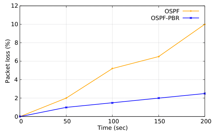
Figure 4. Packet loss comparison in OSPF and OSPF with PBR module.
