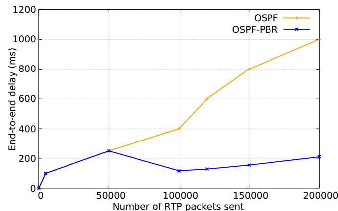
Figure 8. End-to-end delay comparison in OSPF and OSPF with PBR module.
